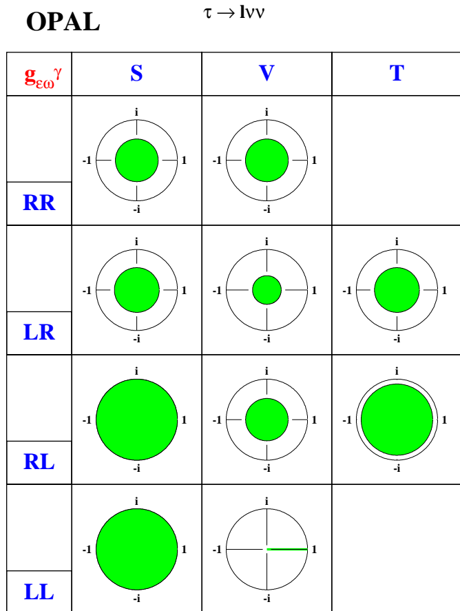
Fig. 7. 90% confidence limits on the normalized coupling constants g_{\epsilon\omega}^\gamma/g_{\max}^\gamma (with g_{\max}^S = 2 , g_{\max}^V = 1 and g_{\max}^T = 1/\sqrt{3} ) under assumption of e\text{-}\mu universality. The Standard Model coupling g_{LL}^V which is not constrained is chosen to be real and positive
