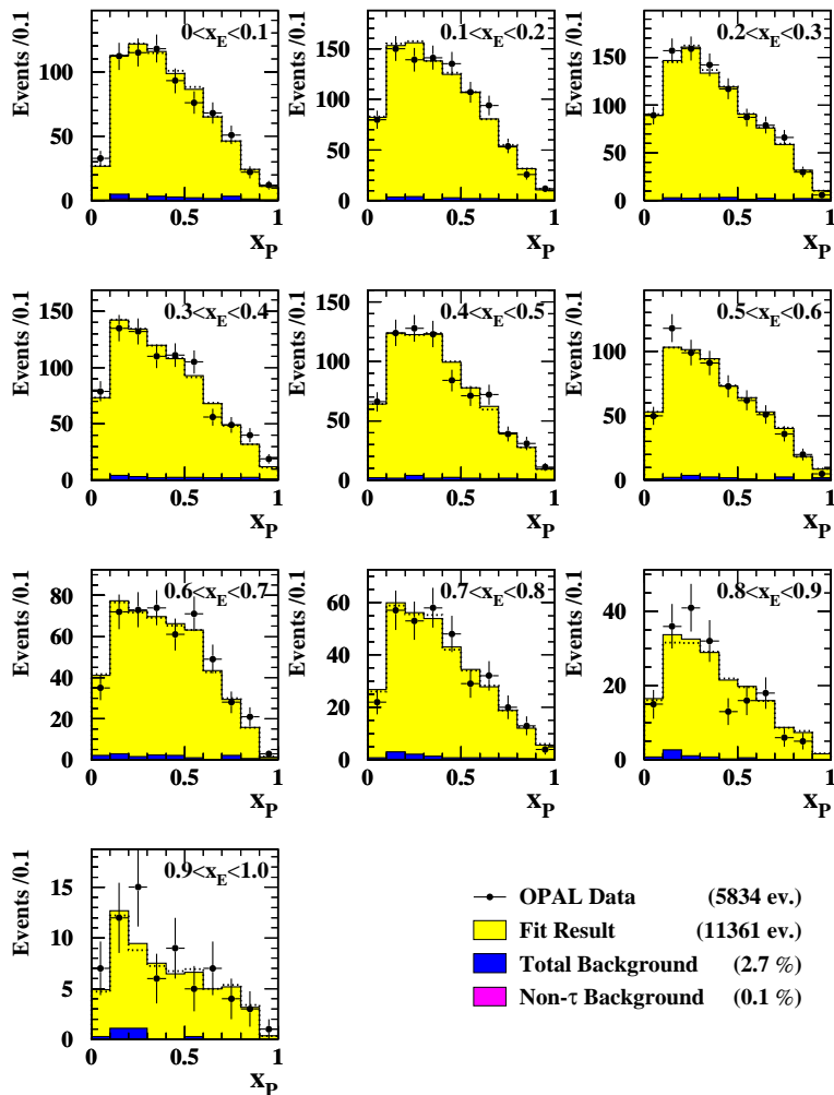
Fig. 5. The correlated \tau \rightarrow e\nu_e\nu_\tau and \tau \rightarrow \mu\nu_\mu\nu_\tau decay spectra from e-\mu events together with the Monte Carlo distribution from the global fit. The spectrum of the scaled momentum, x_p , of the decay muon is shown in slices of each bin of the scaled electron energy, x_E . The dotted line represents the Standard Model expectation. (The plots show the same bins as figure 4 in a different order)
