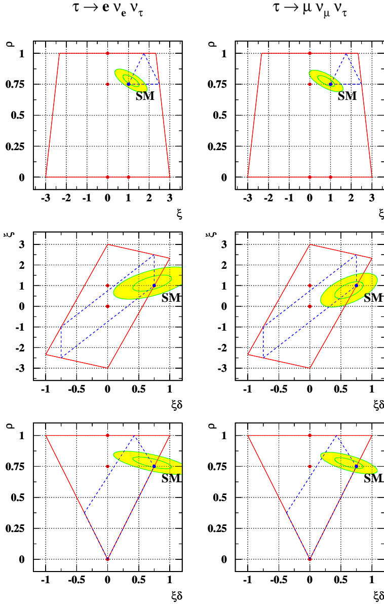
Fig. 6. Presentation of the global fit result in 2-dimensional projections of the Michel parameter space. Shown are the 1 and 2 \sigma ellipses of the fitted parameters. The outer (solid) line encloses the physically allowed region of the parameters. The dashed line confines the area that remains when the parameter which is not plotted is fixed to its Standard Model value. The closed circles indicate the basis spectra used in the fit. The labeled one represents the Standard Model
