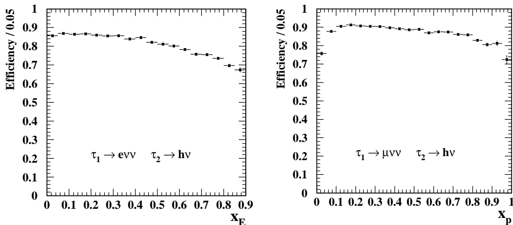
Fig. 1. Selection efficiencies for the e-h ( \mu -h) event samples as a function of the scaled lepton energy (momentum), x_E ( x_p ), as determined from the Monte Carlo after the preselection including all fiducial cuts
